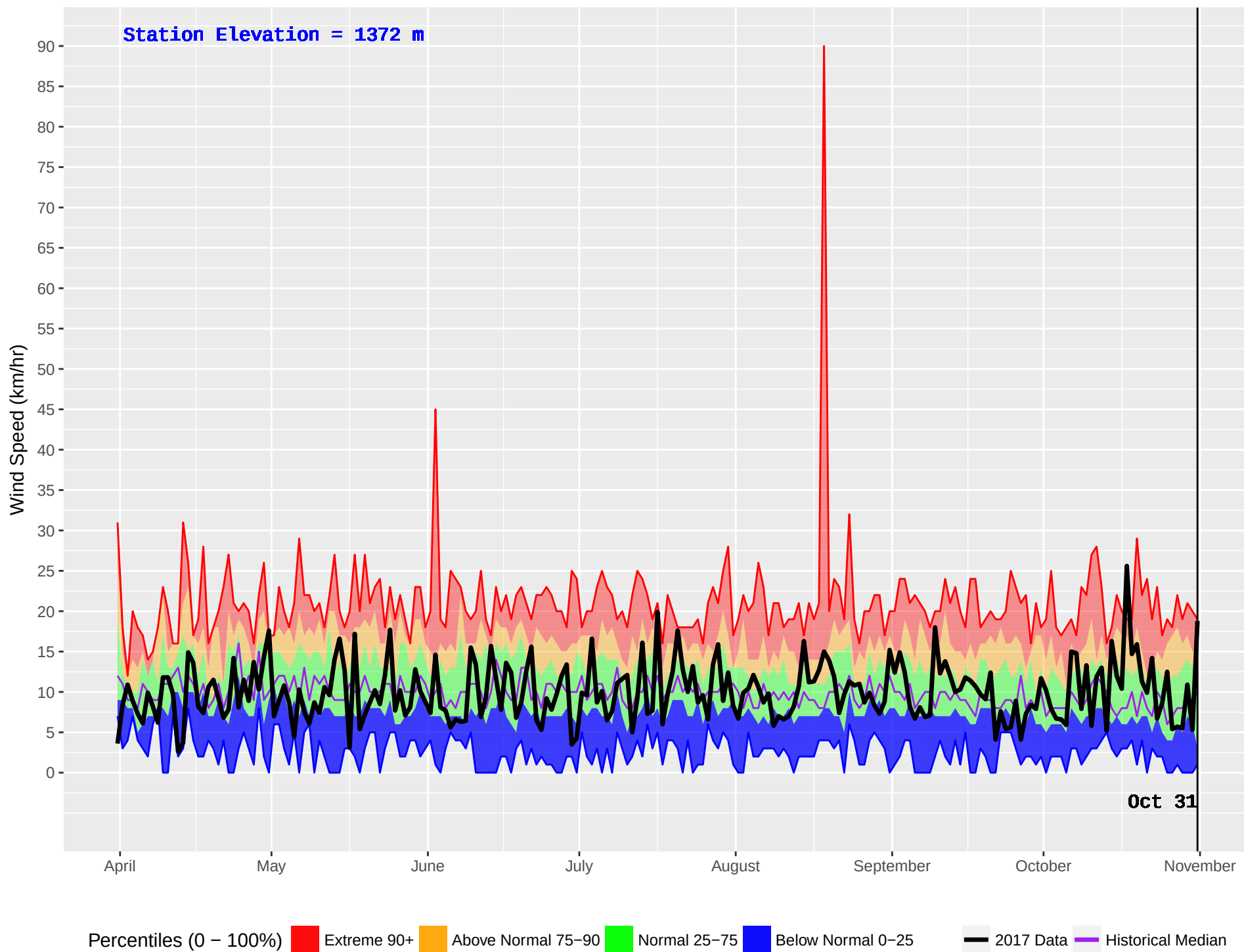
CHERRY LAKE (791) : Historical (1989–2016) and Current (2017) Noon Wind Speed
